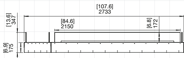
104BN.BX1 (LEFT DECORATIVE BOX)
