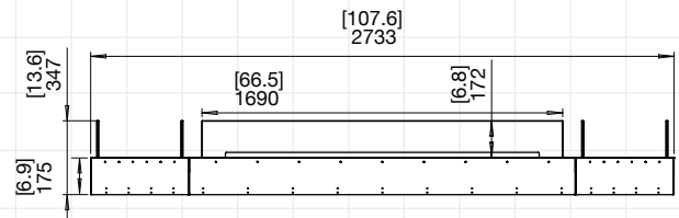
104BN.BX2 (LEFT & RIGHT DECORATIVE BOXES)
